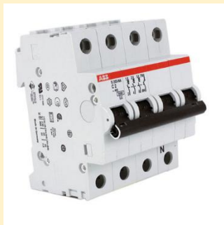
MCB
